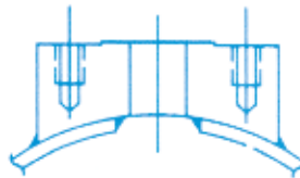
OUTSIDE RADIUS MOUNT
