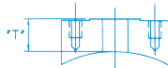
FOR CYLINDRICAL RADIUS MOUNT
